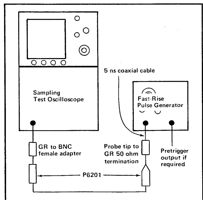
Fig. 5-7. Equipment setup for steps 7 and 8.
