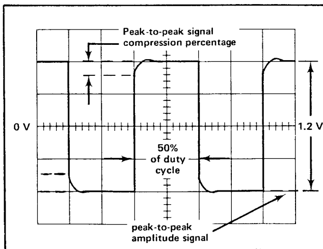
Fig. 5-6. Illustration showing how to measure signal compression.
