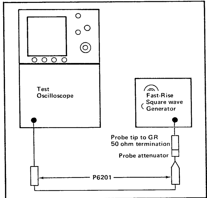
Fig. 5-8. Equipment setup for step 9.
