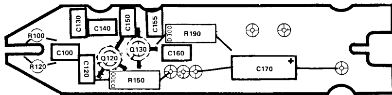
PROBE-FET (FRONT)
