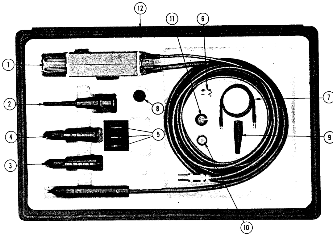
Fig. 1-1. P6201 Probe and Standard Accessories.
